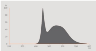
LISO spectral power distribution 6500K CRI80 v1
