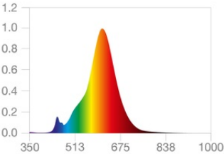
EPREL Data Spectral Diagram LEDr AC42295 2200K TW
