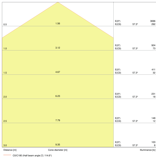
PANEL D | 1200 36W 4000K UGR19
