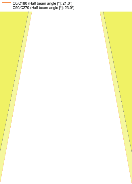
TRACK SP D85 35W4000K 90RA NFL BK
