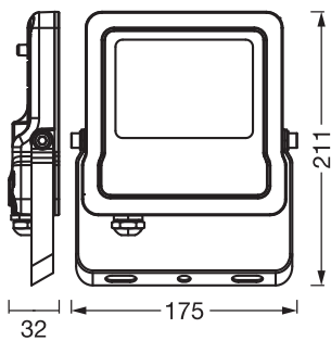
SMART WIFI MAT FLOOD 30W RGBW LEDV
