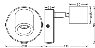
LED SPOT BRICK 1XGU10 WT
