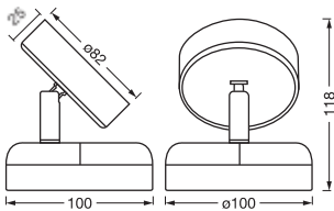
NIGHTLUX ROUND 830 DIM USB BK
