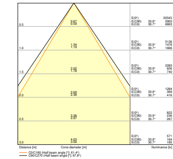
LB FLEX 1200 P 42W 840 N WITH BP COVER
