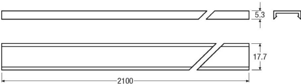
Clean Cover LF-LTS-COVER-C Order code 4008321790187
