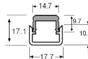
Slim Track + Diffuse cover LF-LTS-COVER-S (for LF800S)
