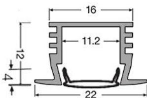
Slim Track + Slim cover frosted matte FX-QMS-G1-CFDB-300
