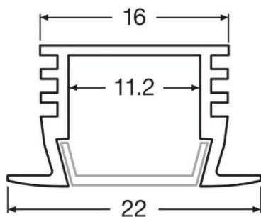
Slim Track FX-QMS-G1-TU16H12W3-300 Order code 4052899448988
