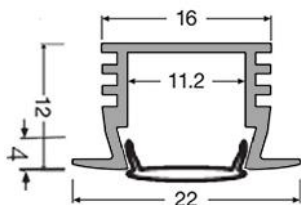
Slim Track + Slim cover frosted FX-QMS-G1-CFDL-300
