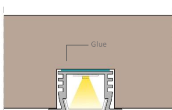
Application example with glue on wood
