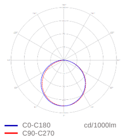
Slim cover frosted
