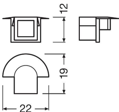
Plastic End cap grey plain FX-QMS-G1-EFGP-TU16H12W3 Order code 4052899449817
