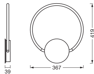
DECOR AURA WALL 10W 830 CLICK SEL
