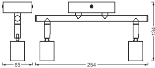
LED SPOT CYLINDER 2XGU10
