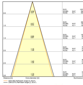
UB WL VARIO RD 29W ML 822 BK 30D Up Down
