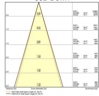
UB WL VARIO RD 29W ML 827 BK 55D Up Down
