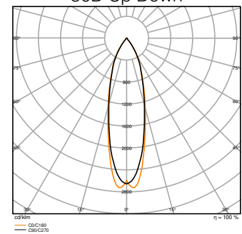
UB WL VARIO RD 29W ML 822 BK 30D Down
