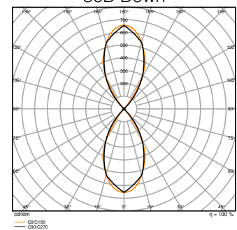
UB WL VARIO RD 29W ML 822 BK 55D Up Down
