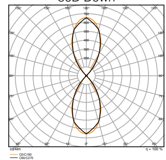
UB WL VARIO RD 29W ML 822 GY 55D Up Down
