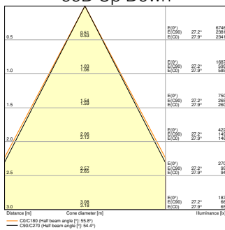
UB WL VARIO RD 29W ML 827 GY 55D Up Down
