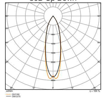
UB WL VARIO RD 29W ML 822 GY 30D Up Down
