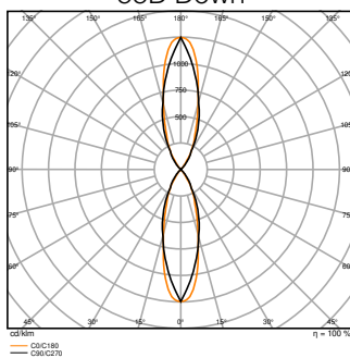
UB WL VARIO RD 29W ML 822 GY 30D Up Down
