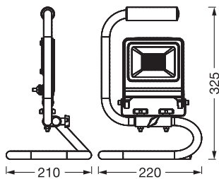
LED WORKLIGHT 30W S-STAND CH PLUG OSRAM
