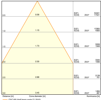
HB DA P 75W 840 70DEG IP66 WITH REFRACTOR
