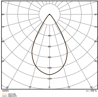
HB DA P 75W 840 70DEG IP66 WITH REFLECTOR
