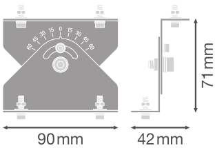
LB FLEX ANGULATION MOUNT KIT
