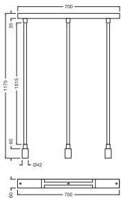
DECOR GLOW PEND LN3XE27 LED SELECT
