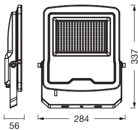
ENDURA FLOOD PCR 100W 840 DG
