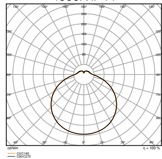
SF SQUARE 330 V 24W 3CCT 5000K IP44
