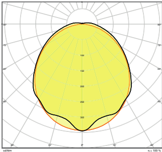
DampProofLED 1200 39W 6500K IP65
