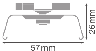
TRUSYS PFM TRUSYS FLEX GRID CEILING CLIP
