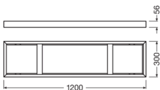
PANEL 1200 SURFACE MOUNT KIT
