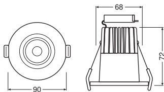
707988_LEDVANCE Spot-FP LED fix 7W
