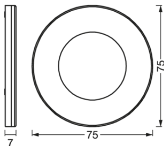
UNDERCABINET SPOTMAGNET
