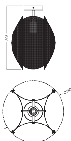
DECOR FOLDED GLOBE CEILING E27 GD
