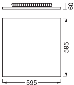
PLANON FRAMELESS 600X600 40W 830
