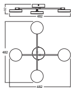
DECOR SPOT MOON 4SP CROSS 21W 830BK
