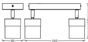
LED SPOT HALF WOOD LINE 2XGU10 WT
