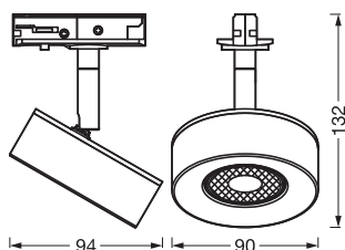
TRACKLIGHT SPOT BEAM 4.8W
