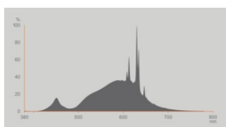
Spectral graph Classic 2700K
