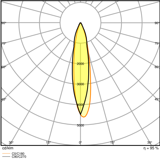
LEDVANCE FLOODLIGHT SYM 190W 20D
