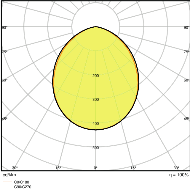
Floodlight LED 50W 4000K BK S IP65
