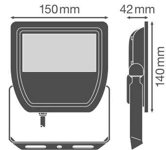
FLOOD LED 30W BK 100 DEG IP65
