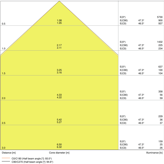
FLOOD LED 30W 3000K BK 100DEG IP65
