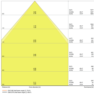
Panel LED 1200 33W 4000K 230V UGR19
