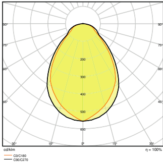
4058075807280 Panel LED 1200 33W 4000K 230V UGR19
