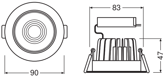
707987_LEDVANCE Spot LED adjust 8W
