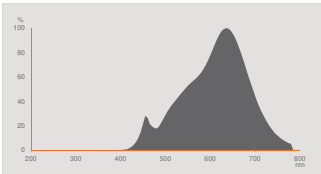
CITIZEN 1202C4 V6 2700K
