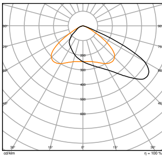
FL FLEX P 80W ML 820 A55X120 WAL LEDV
