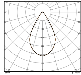
HB DA P 75W 840 70DEG IP66 WITH REFRACTOR
