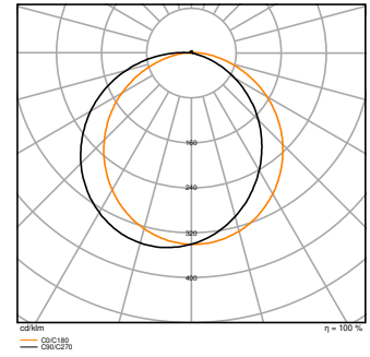
BLKH RD 250 P 9.5W 830 CPS BK with Eyelid
