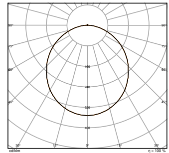
BLKH 250 P 10W 840 1200lm
