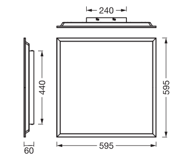
PANEL ESSENTIAL 60X60 36W840 WT
