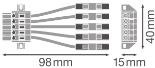
TRUSYS FLEX FEED IN CONNECTOR 5P
