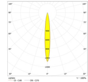
FL H M LUM V 300W/500W SYM R12
