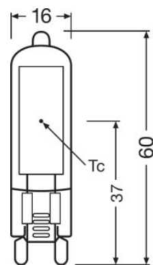
BASE PIN 30 2.8 W/2700K G9
