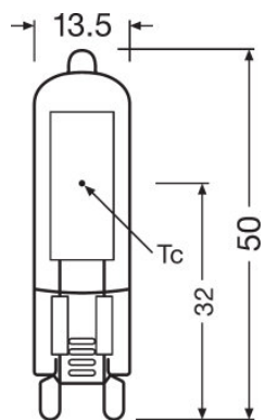
BASE PIN 20 2 W/2700K G9
