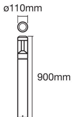
SMART+ MODERN LANTERN Bollard 90cm Multicolor
