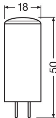
ST PIN 35 320° 3.3 W/2700K GY6.35
