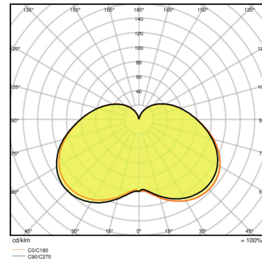
LED STAR STICK 60 FR 8 W/4000K E14
