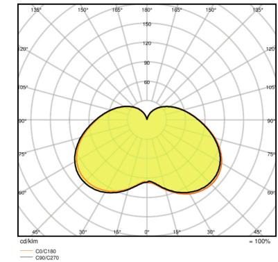
LED STAR STICK 75 FR 10 W/2700K E14
