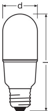
LED STAR STICK 60 FR 8 W/2700K E27, LED STAR STICK 60 FR 8 W/4000K E27, LED STAR STICK 75 FR 10 W/2700K E27, LED STAR STICK 75 FR 10 W/4000K E27
