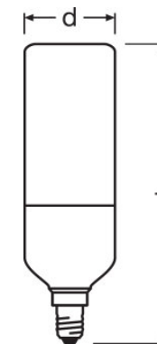
LED STAR STICK 0.5 W/1500K E14
