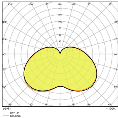
LED STAR STICK 60 FR 8 W/2700K E14
