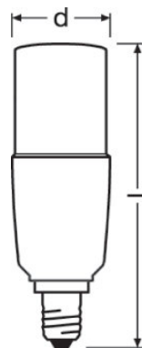
LED STAR STICK 60 FR 8 W/2700K E14, LED STAR STICK 60 FR 8 W/4000K E14, LED STAR STICK 75 FR 10 W/2700K E14, LED STAR STICK 75 FR 10 W/4000K E14
