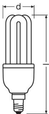
D STICK 11 W/2700K 220...240 V E14, D STICK 11 W/4000K 220...240 V E14, D STICK 11 W/6500K 220...240 V E14
