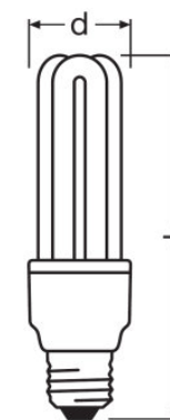
D STICK 15 W/2700K 220...240 V E27, D STICK 15 W/4000K 220...240 V E27, D STICK 15 W/6500K 220...240 V E27
