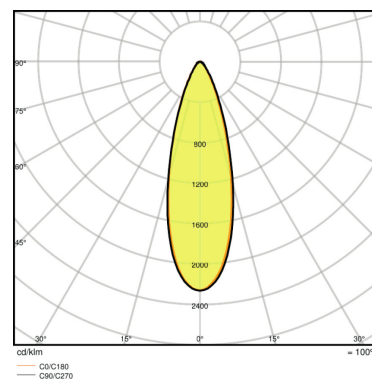
P PAR30 DIM 75 36° 10.5 W/2700K E27
