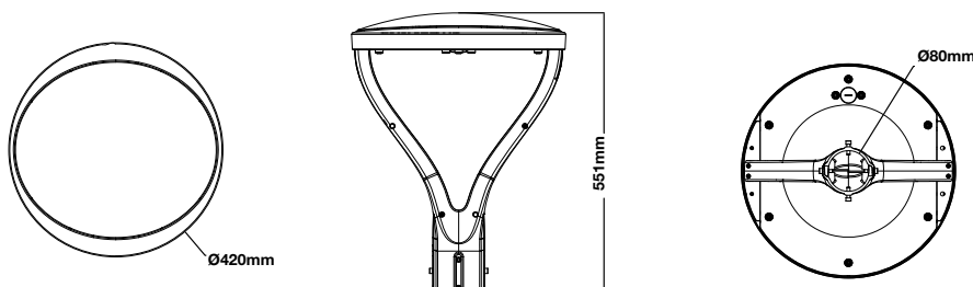
LPT100MWTC 100/75/50/30W Diameter Ø420mm x H 551mm Flex fit for 73-78mm pole
